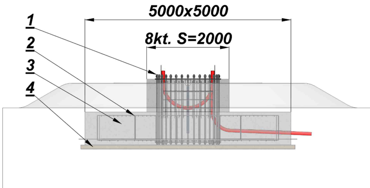
Fig.16. Overall dimensions of the exemplary foundation for the ZEFIR D14-P10-T23 turbine set.
