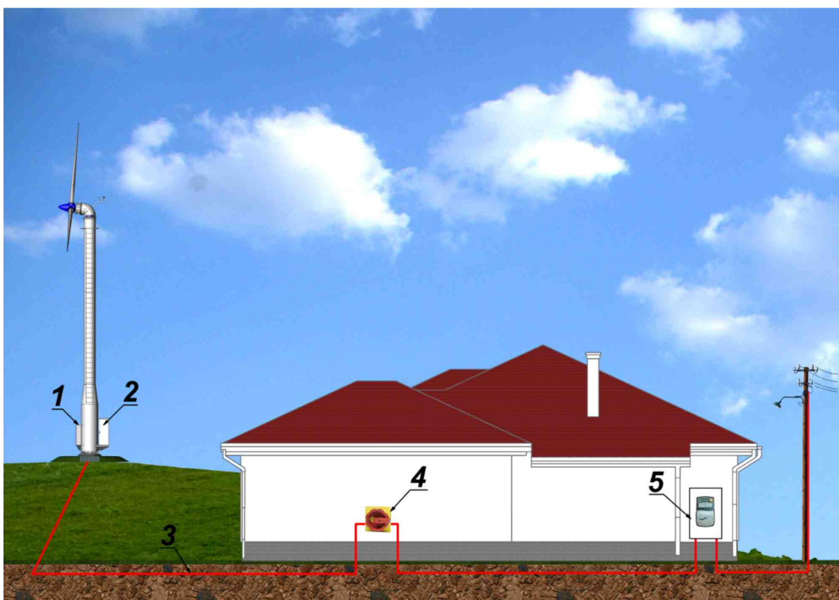
Fig.22. Wiring diagram of the ZEFIR D14-P10-T23 power plant working in on-grid system with inverter located on the tower of the power plant. 1-power plant control cabinet, 2- the inverter, 3- cable link from the power plant to the building, 4- switch, 5- electric meter
