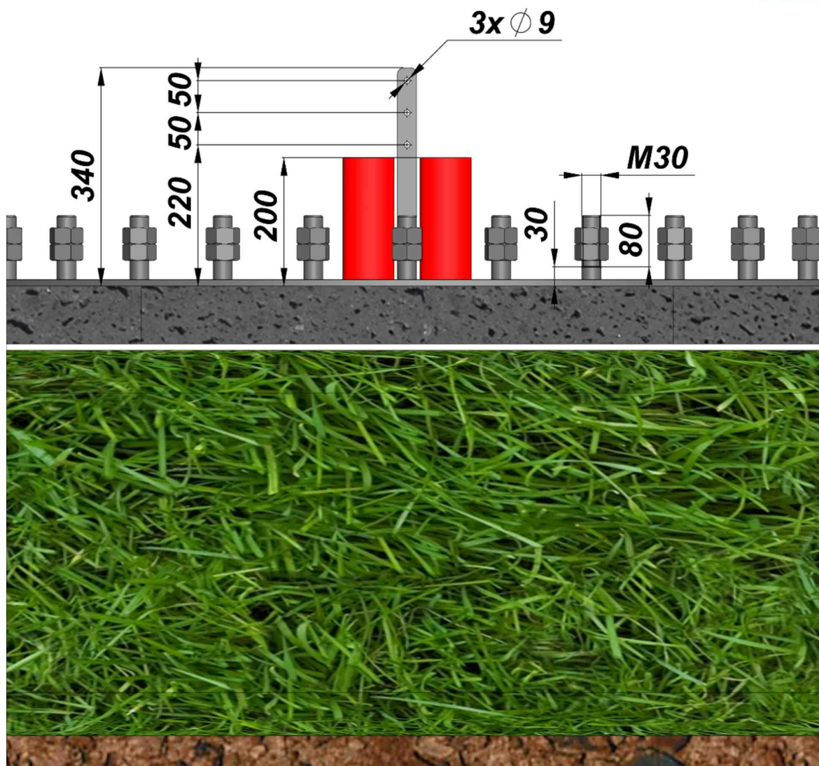
Fig.7. Grounding and protective pipes lead out from the ZEFIR D14-P10-T23 turbine set foundation.
