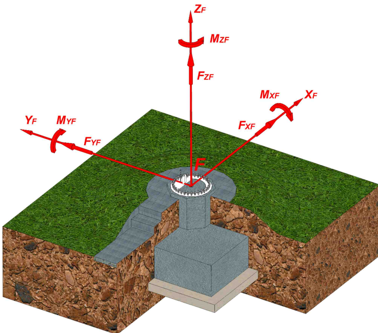
Fig. 11. The coordinate system to determine ZEFIR D14-P10-T23 wind turbine foundation loads.
