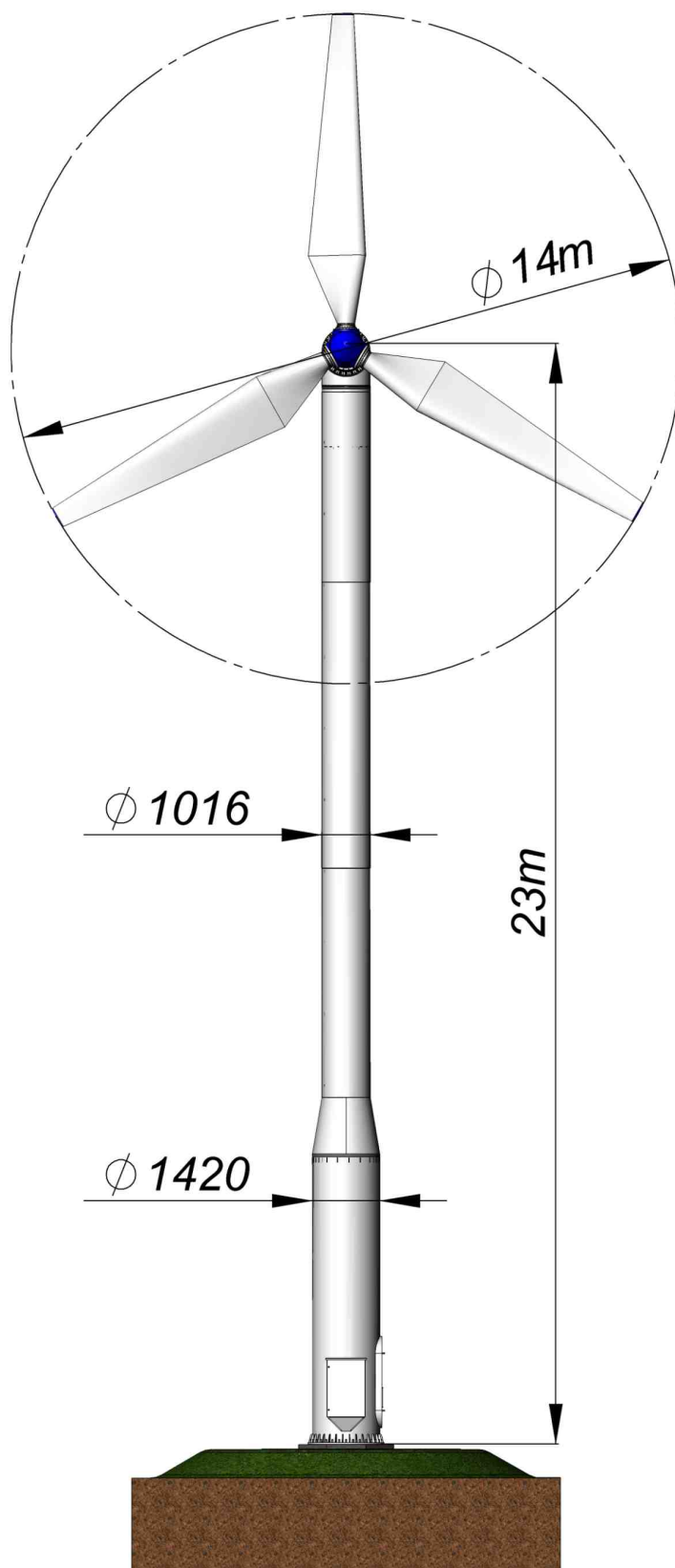
Fig.1. ZEFIR D14-P10-T23 wind turbo-generator. Front view.
