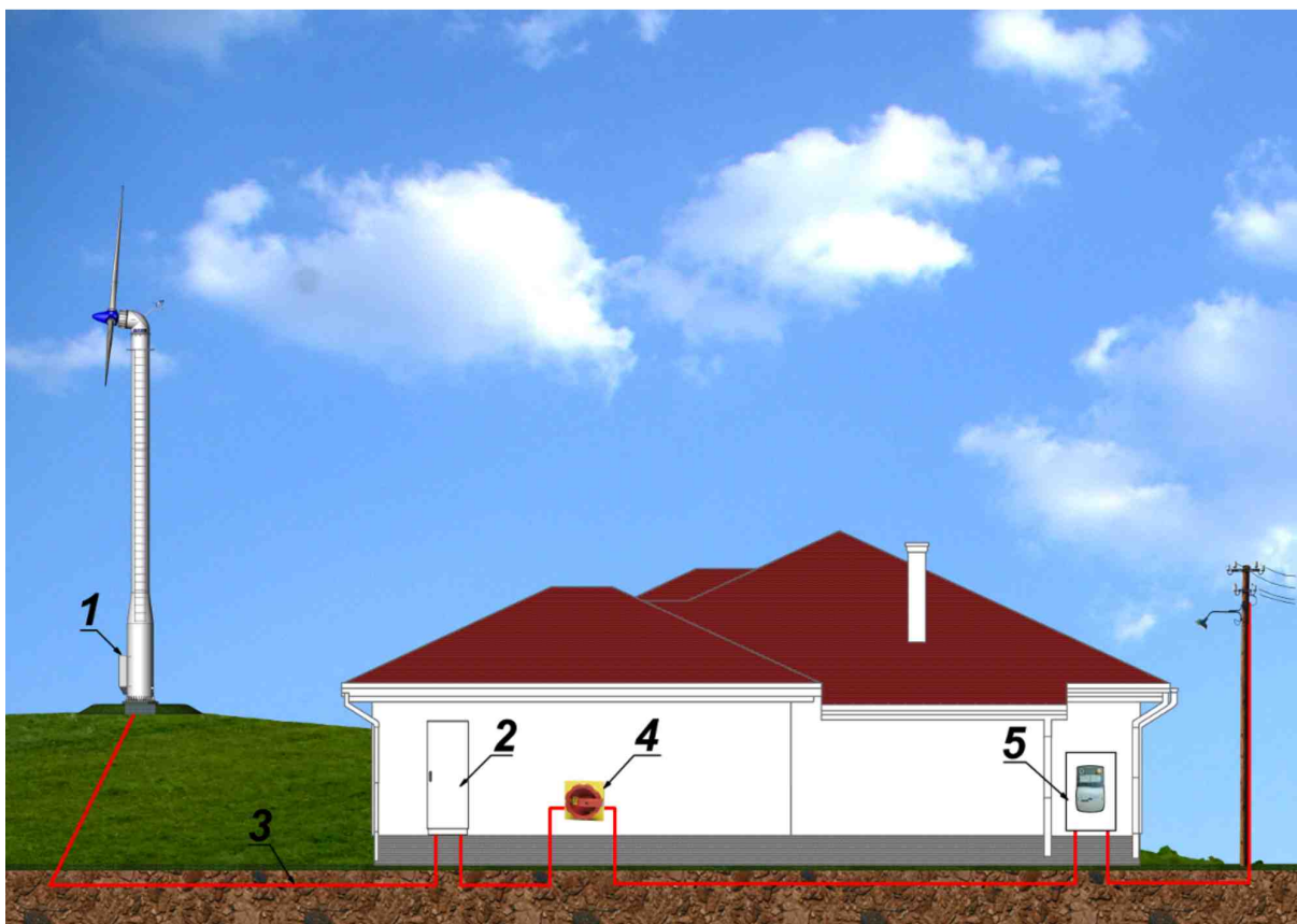
Fig.23. Wiring diagram of the ZEFIR D14-P10-T23 power plant working in on-grid system with inverter located in the building. 1- power plant control cabinet, 2- the inverter, 3- cable link from the power plant to the building, 4- switch, 5- electric meter
