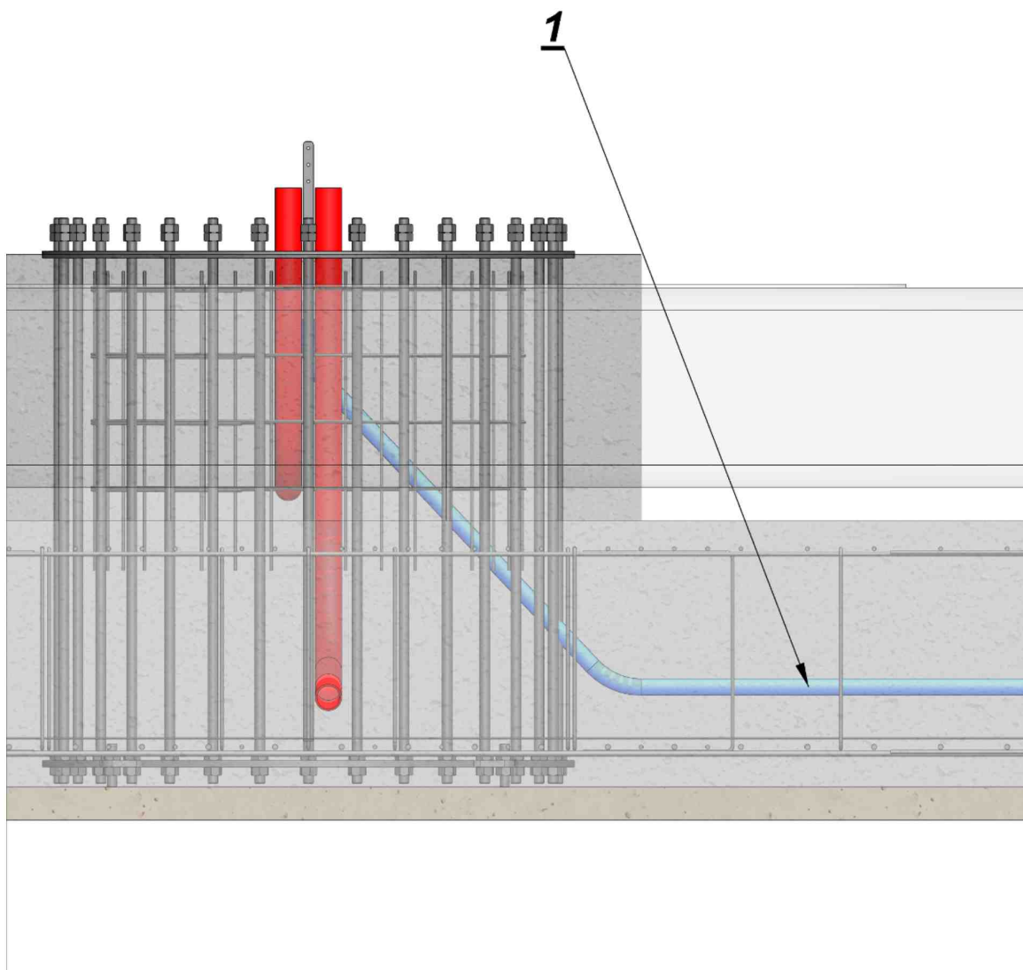
Fig.10. Grounding bar and protective pipes led out from the ZEFIR D14-P10-T23 turbine set foundation.
