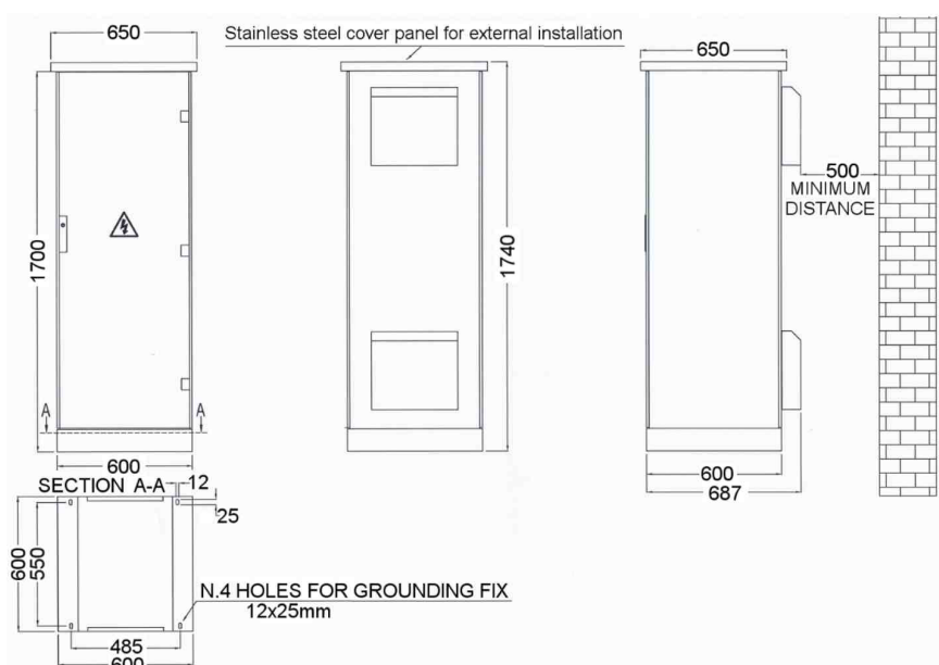
Fig.24. Installation conditions of the CLEANVERTER 10TL inverter in the building.
