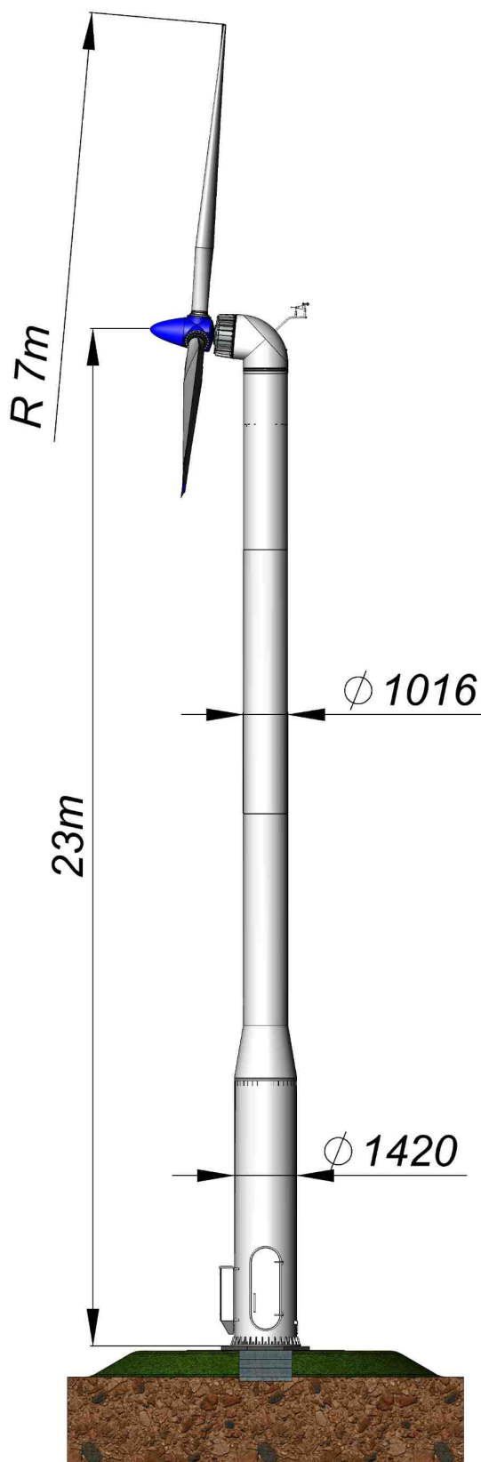
Fig.2. ZEFIR D14-P10-T23 wind turbo-generator. Side view.
