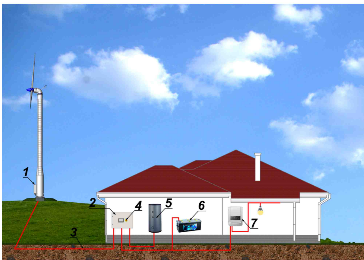
Fig.25. ZEFIR D14-P10-T23 power plant off-grid wiring diagram with the load generator in the building.
